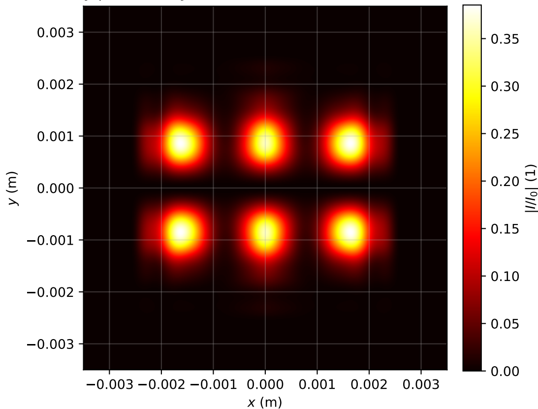
Intensity profile I(x, y, z = 3.582)/I_0 , P_{in}=3.0P_{cr} , artificial time
